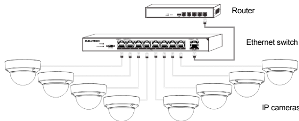
Figure 2: Ethernet switch connection diagram
