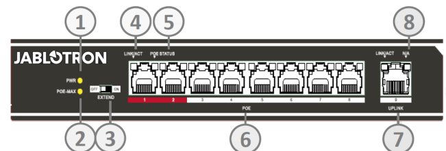
Figure 4: Front panel of the switch: 1 – power supply indicator; 2 – PoE power supply overload indicator; 3 – "EXTEND" switch to boost the PoE power supply to increase the maximum LAN cable length; 4 – LAN device activity indicator; 5 – PoE power supply use indicator; 6 – RJ-45 connectors for IP cameras with PoE power supply; 7 – RJ-45 connector for router connection; 8 – no function
